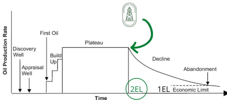
A theoretical oil & gas well production curve showing when the AWA must collect to fund decommissioning
